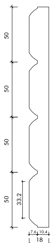
D 50-16R Scale - NTS
