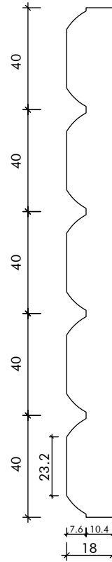
C 40-16R Scale - NTS
